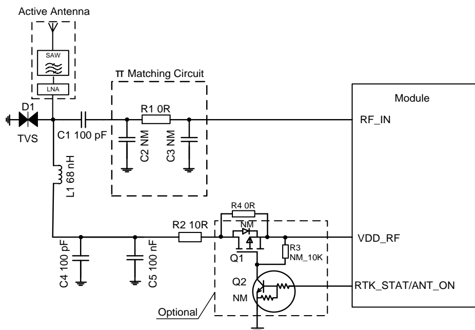
Figure 17: Active Antenna Reference Design
