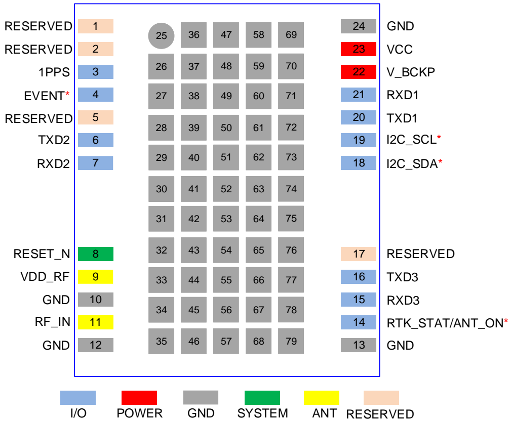
Figure 3: Pin Assignment
