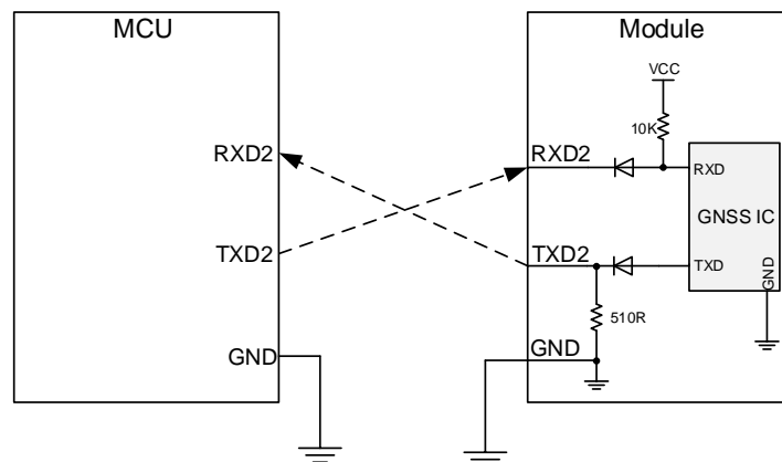
Figure 12: UART2 Interface Reference Design
