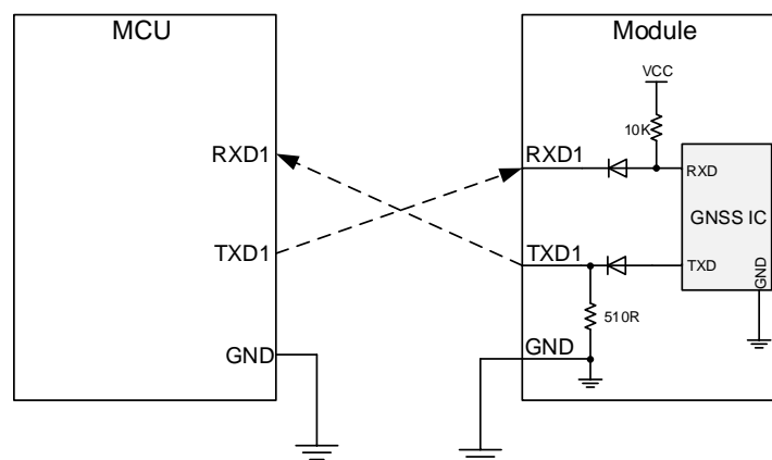
Figure 11: UART1 Interface Reference Design
