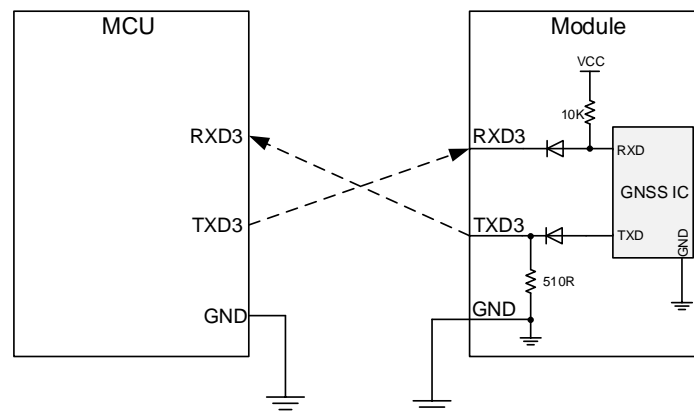
Figure 13: UART3 Interface Reference Design
