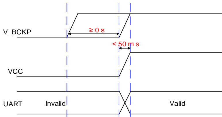
Figure 9: Power-up Sequence
