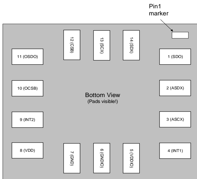
Pin-out bottom view
